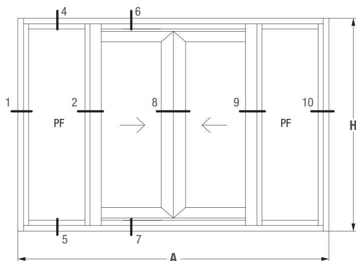
SECCION 2-8-9-10
